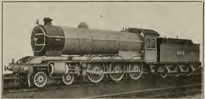
THREE-CYLINDER PACIFIC FREIGHT LOCOMOTIVE ON THE NORTH EASTERN RAILWAY—ENGLAND.
